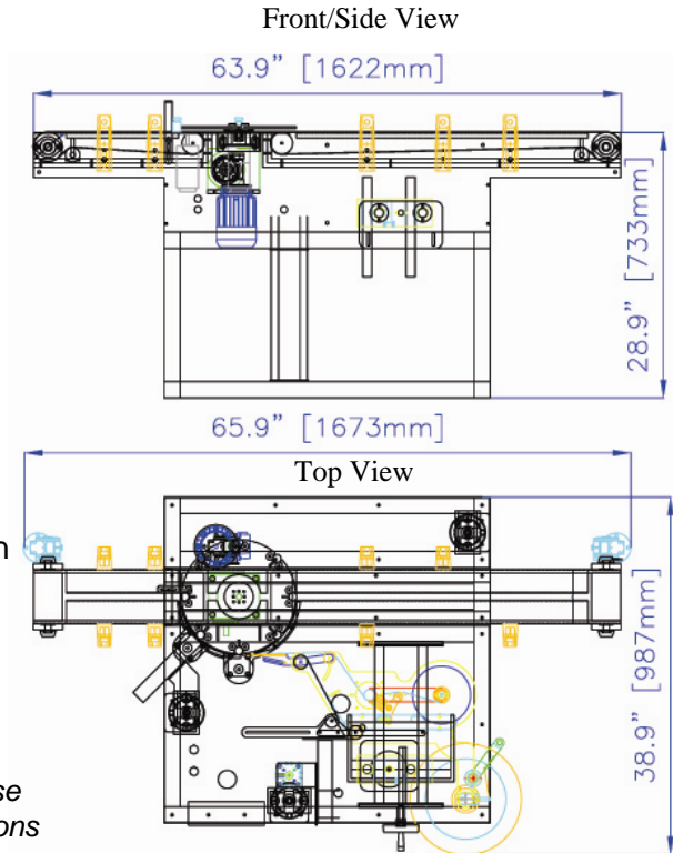
Dimensional Drawing
