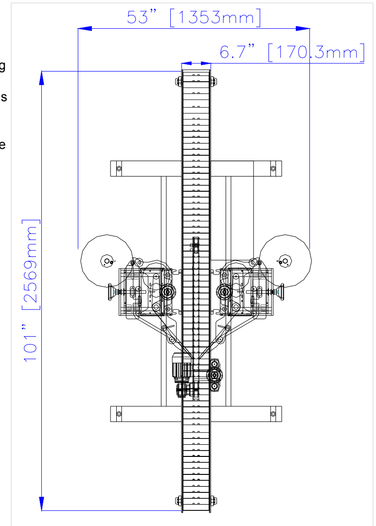
Dimensional Drawing
